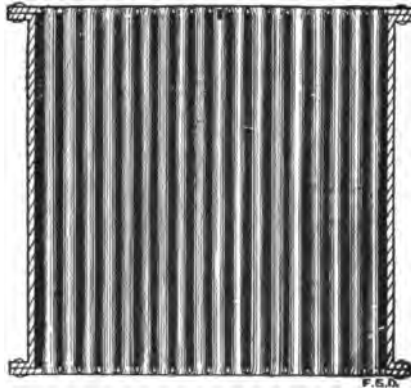
FIG. 144.—Copper Shell and Flue Boiler, with flange connections for the tube plates, as used on the "Locomotive" and other American steam carriages. The shell is strengthened by winding several layers of steel piano wire around the length of the boiler. This cut gives a section on the centre, showing one row of flues.
